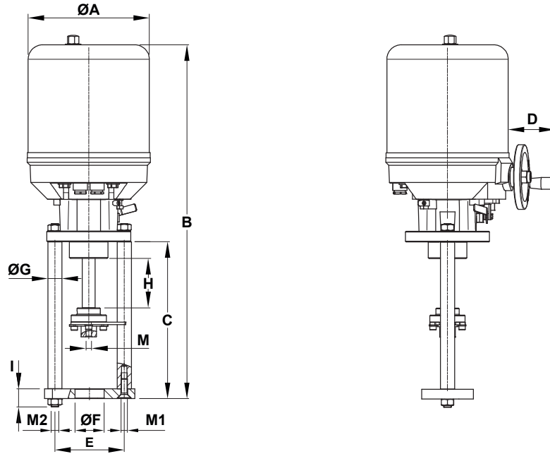
DIMENSIONS (mm)
